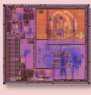
Vivosoc4 – SMIC130 4x RI5CY
