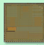
Kosmodrom – GF22 2x Ariane + 3 RI5CY
