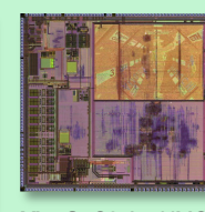
VivoSoC3.1 – UMC180 4x Or1k
