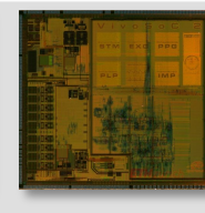
Vivosoc3 – SMIC130 4x Or10n
