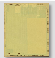
Vega – GF22 10x RI5CY
