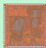
Atomario – UMC65 8x RI5CY
