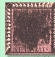
Artemis – UMC65 4x Or10n
