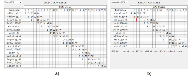
Figure 2: Pipeline diagram in both visualization methods: (a) ‘Full loops’ and (b) ‘squashed loops’.
