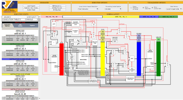
Figure 1: WebRISC-V main page.
